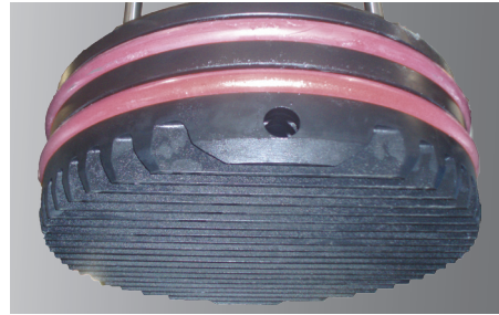
Finned or flat platens better adapt to various adhesive types. All platens are Teflon® coated and include cast-in heaters.
